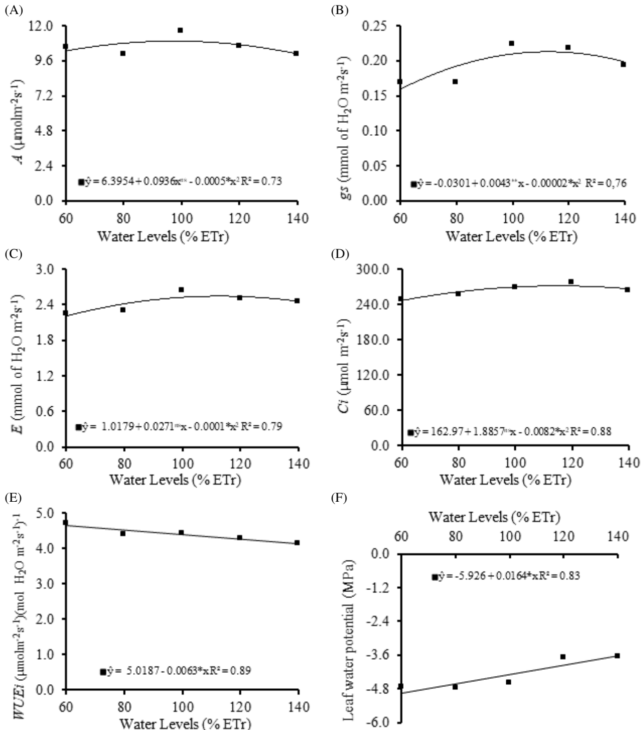
Figure 1. \text{CO}_2 assimilation rate - A (A), stomatal conductance - g_s (B), transpiration - E (C), internal \text{CO}_2 concentration - C_i (D), intrinsic water use efficiency - WUE_i (E) and leaf water potential (F) of Annona squamosa L. seedlings as a function of irrigation depths at 120 days after treatments began to be applied.
