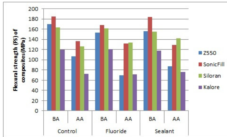
Figure 2. Flexural strength (FS) of composites before aging (BA) and after aging (AA)
