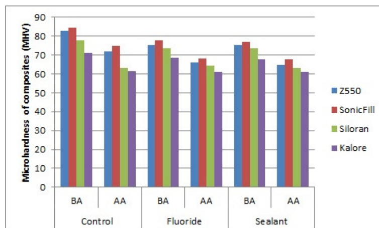
Figure 3. Microhardness of composites before aging (BA) and after aging (AA)
