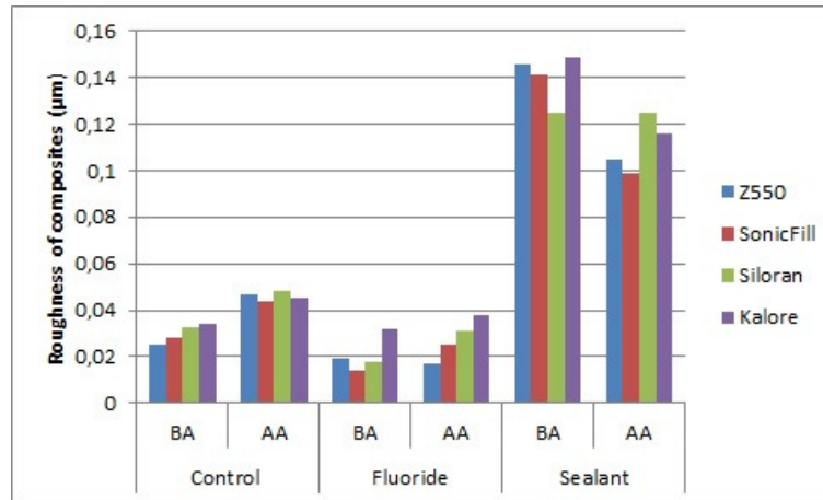
Figure 4. Roughness of composites before aging (BA) and after aging (AA)
