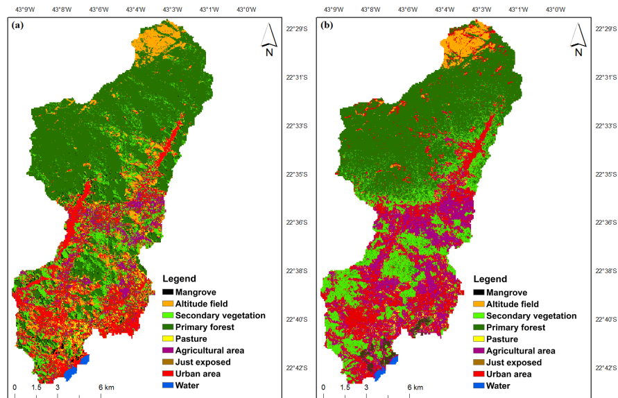
Figure 3. Classes of land use and coverage for 2005 (a) and 2010 (b) by the maximum likelihood method in the Roncador River basin.
