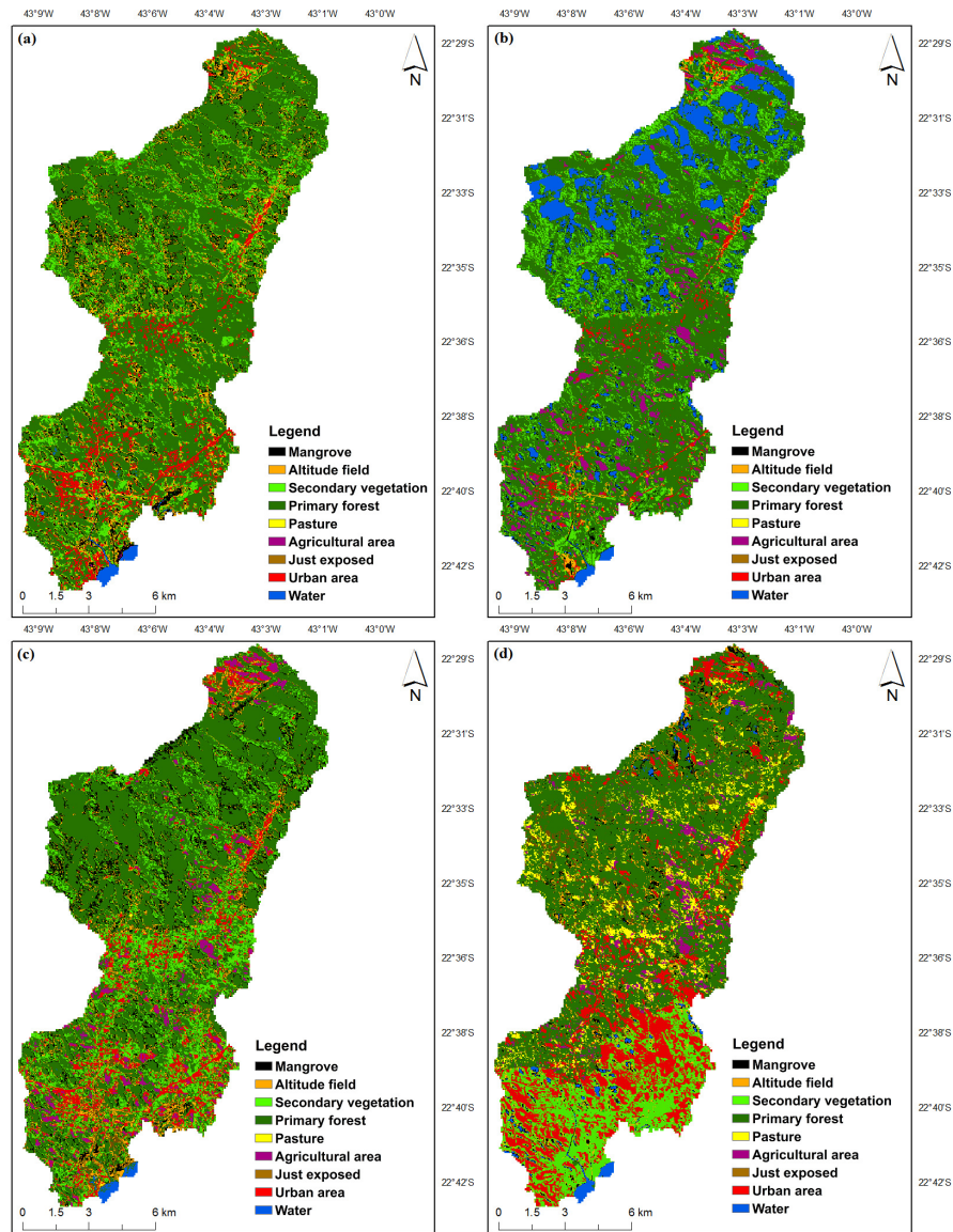
Figure 2. Classes of land use and occupation for the years 1985 (a), 1990 (b), 1995 (c) and 2000 (d) by the K-Means method in the Roncador River basin.
